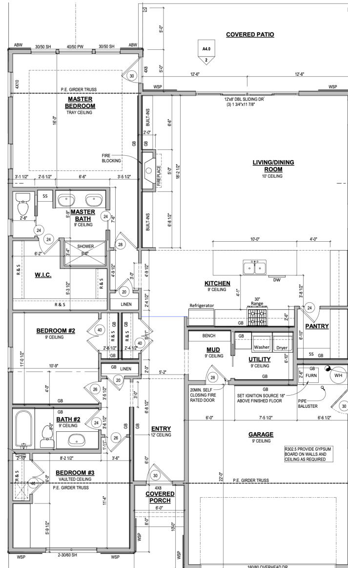
FLOOR PLAN
