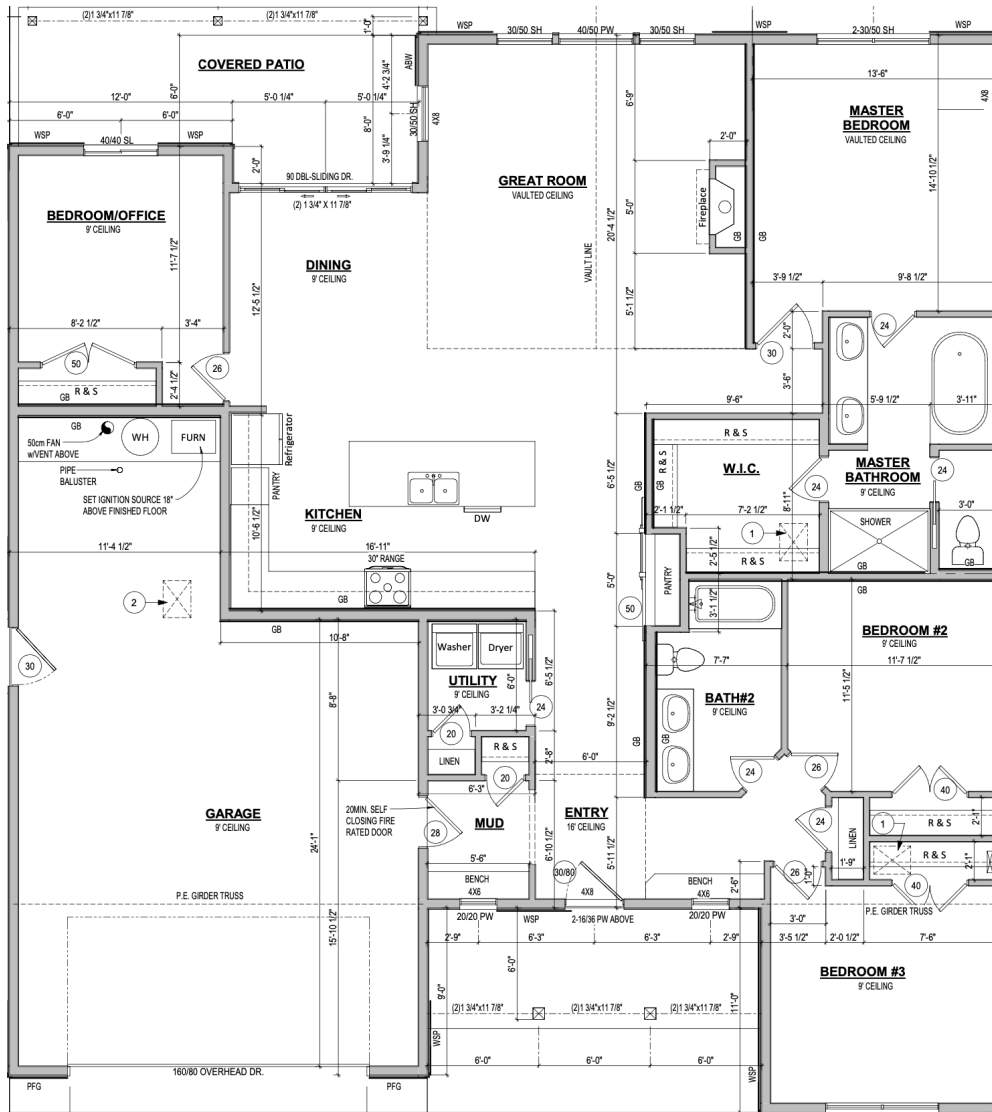
FLOOR PLAN
